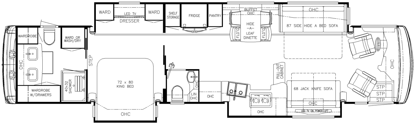
2025 Dutch Star Diesel Pusher 4325
