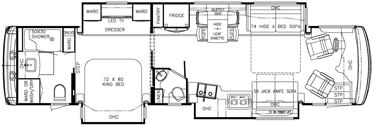
2024 Dutch Star Diesel Pusher 3836
