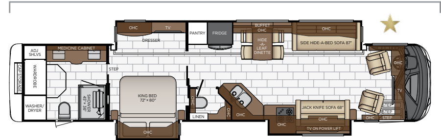
Length: 44' 10"
