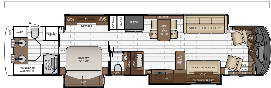
Length: 44' 10"
