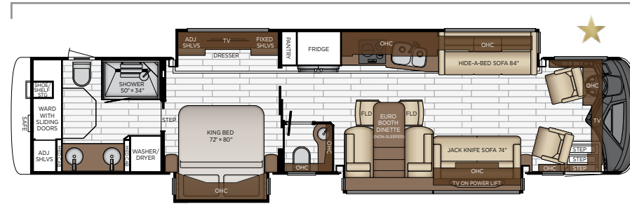
Length: 44' 10"
