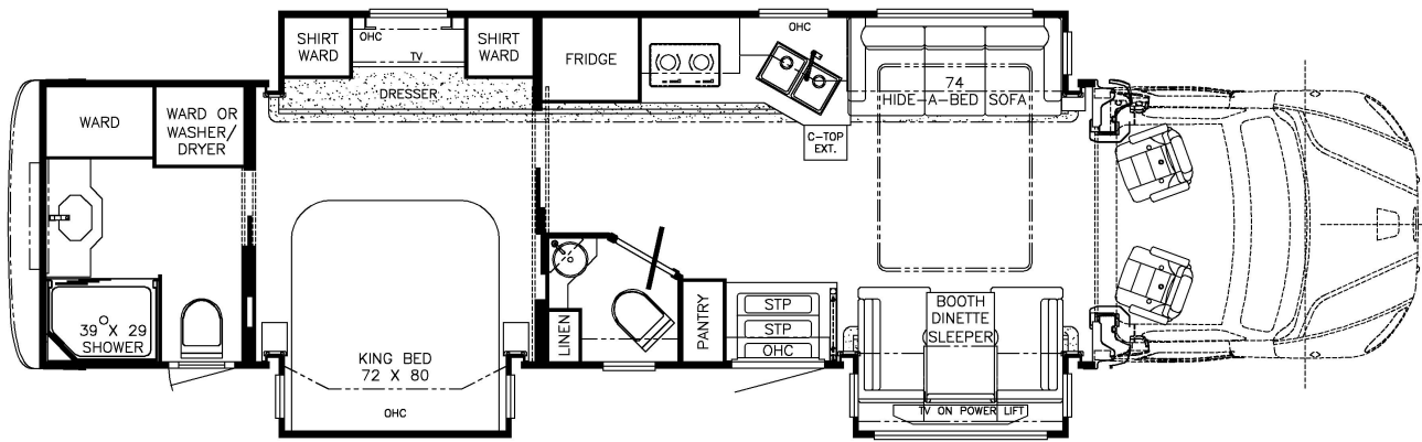
2023 Super Star Super C 4059
