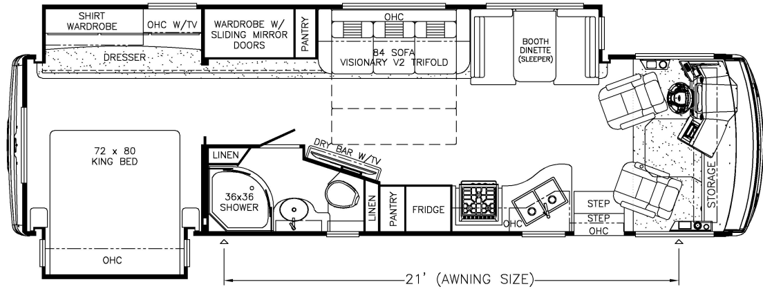
2023 Bay Star Gas Motorhome 3401
