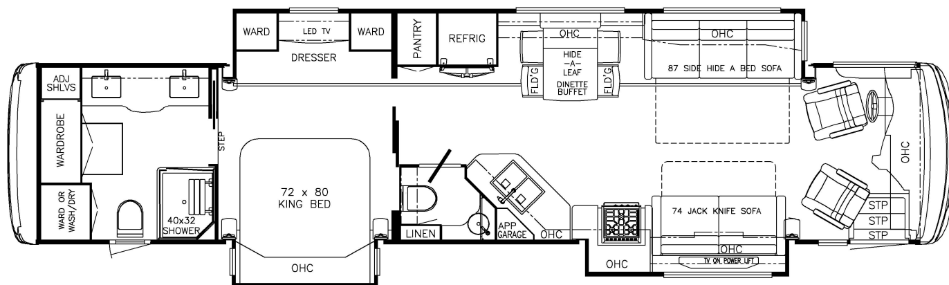
2022 Dutch Star Diesel Pusher 4328
