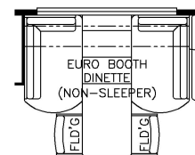
K550 - EURO BOOTH DINETTE (NON-SLEEPER)
