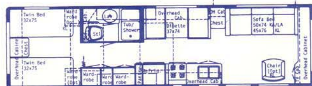
33' Center Bath Dinette • Available Options D, Q, S, F KL, KA, LA
