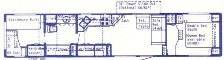
40' Walk Thru Center Bath • Available Option T KL, KA
