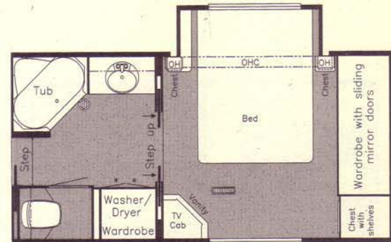
OPTION M445—Cabover S.O. w/sliding doors Available in KAFW 37RDSK, 37RKWB, 38KSWB, 39BRCK, 39BLSE
