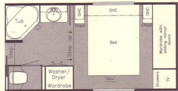
OPTION K343—Honeymoon suite Available in KAFW 37RDSK, 37RKWB, 38KSWB, 39BRCK, 39BLSE
