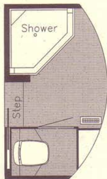
OPTION P094-38" Corner shower ilo tub Available in KAFW 37RDSK, 37RKWB, 38KSWB, 39BRCK, 39BLSE
