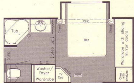
OPTION M615—Cabover S.O. W/80" bed Available in KAFW 37RDSK, 37RKWB, 38KSWB, 39BRCK, 39BLSE
