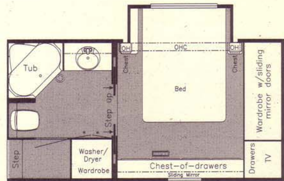
OPTION M442—Cabover S.O. w/dresser center & sliding doors Available in KAFW 38KSSA, 39BRCK
