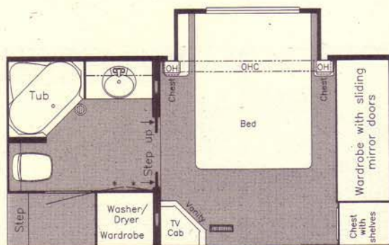
OPTION M446—Cabover S.O. w/sliding doors Available in KAFW 38KSSA, 39BRCK
