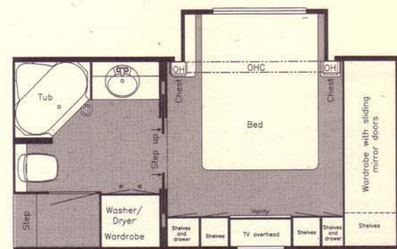
OPTION M447—Cabover S.O. w/vanity center & sliding doors Available in KAFW 38KSSA, 39BRCK
